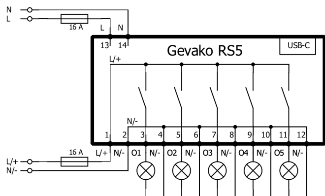
Figure 1: Example application with the RS5
